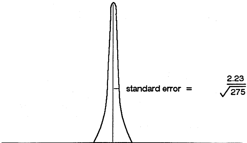
Sampling distribution of \bar{x} 's.
